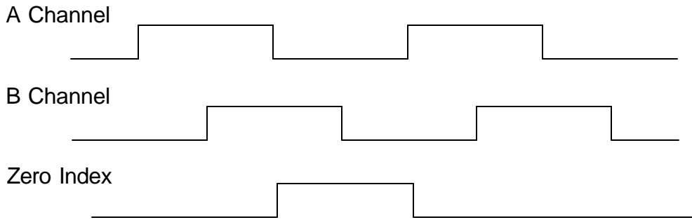
GRAYHILL CW rotation
